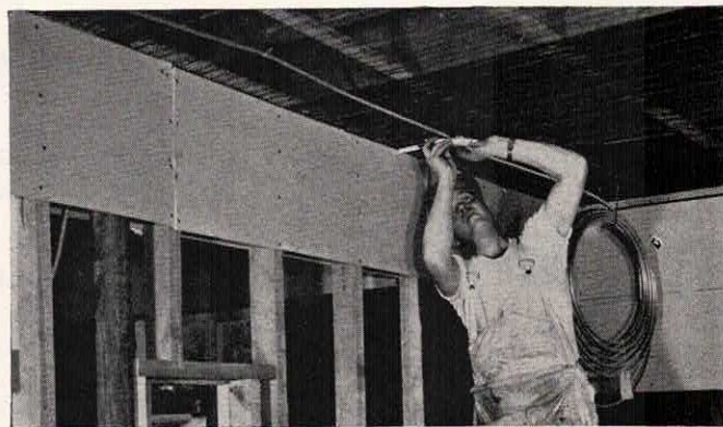
Locating the position of the first tube in the ceiling panel coil. Notice the coil of copper tube temporarily hung from the mesh with a U-hook while the measurement is being taken.
