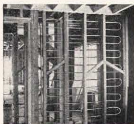
Radiant Heating copper pipes were installed in the dressing-room wall.
