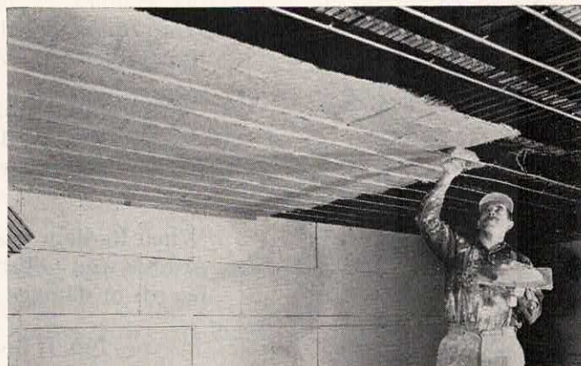
Applying the first or scratch coat of Gypsum plaster to ceiling. Other coats will follow to give final cover of \frac{1}{4} " over copper tube.
