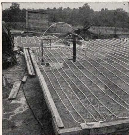
Approximately 1,200 ft. of 3/8" Type L Copper Tube was built into panel coils for this house.
